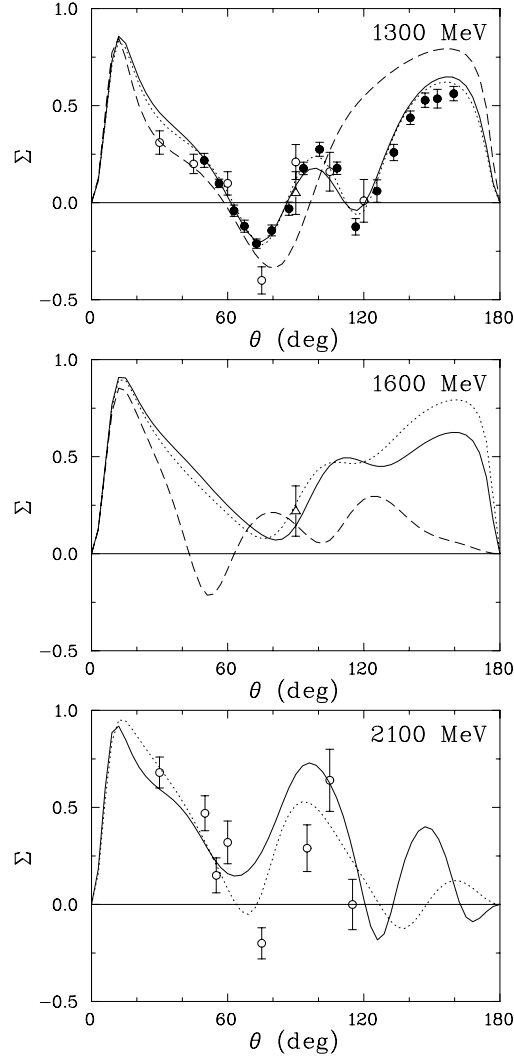
FIG. 10: Beam asymmetry \Sigma for \gamma p \rightarrow \pi^+ n at E_\gamma = 1300, 1600 , and 2100 MeV vs. center-of-mass scattering angle. Solid (dotted) lines correspond to the SAID FA08 (FA07) solution. Dashed lines give the MAID07 [46] predictions. Experimental data are from GRAAL (filled circles) [54], from DNPL (open circles) [55], and from CEA (open triangles) [56]. Plotted uncertainties are statistical. Systematic uncertainties are taken into account in the fit (see text).
