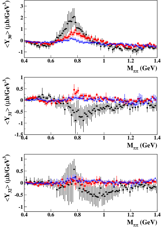
FIG. 6: Moments of the di-pion angular distribution in 3.2 < E_\gamma < 3.4 GeV and -t = 0.45 \pm 0.05 \text{ GeV}^2 (black), -t = 0.65 \pm 0.05 \text{ GeV}^2 (red) and -t = 0.95 \pm 0.05 \text{ GeV}^2 (blue). Error bars include both statistical and systematic uncertainties as explained in the text.
