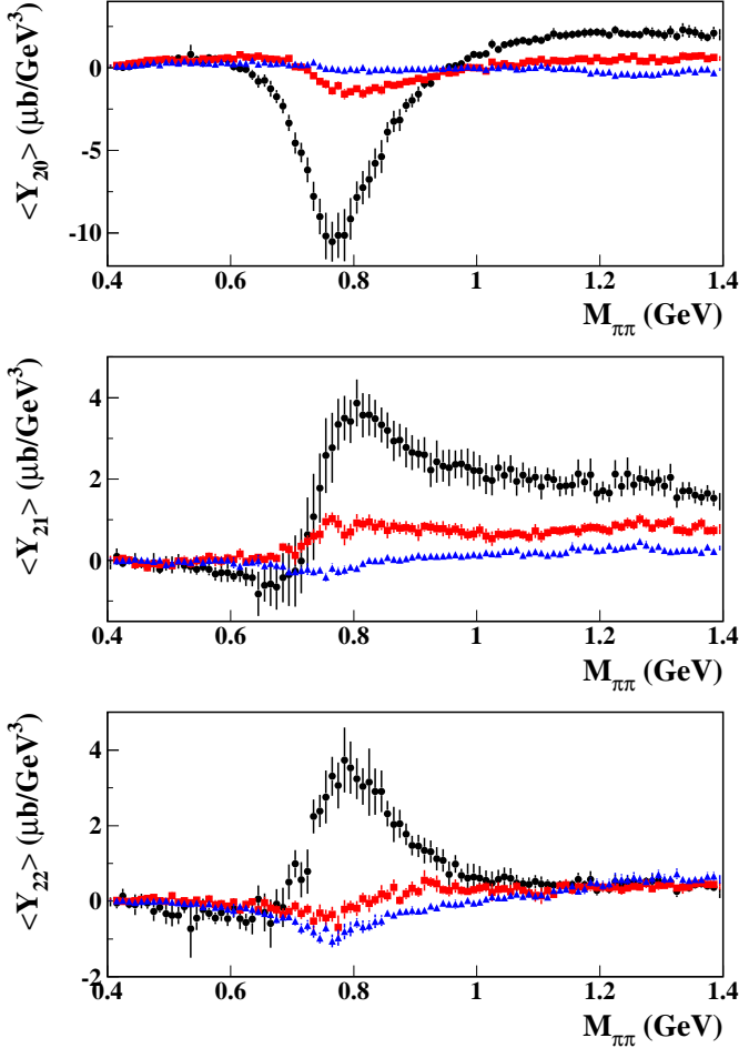
FIG. 5: Moments of the di-pion angular distribution in 3.2 < E_\gamma < 3.4 GeV and -t = 0.45 \pm 0.05 \text{ GeV}^2 (black), -t = 0.65 \pm 0.05 \text{ GeV}^2 (red) and -t = 0.95 \pm 0.05 \text{ GeV}^2 (blue). Error bars include both statistical and systematic uncertainties as explained in the text.
