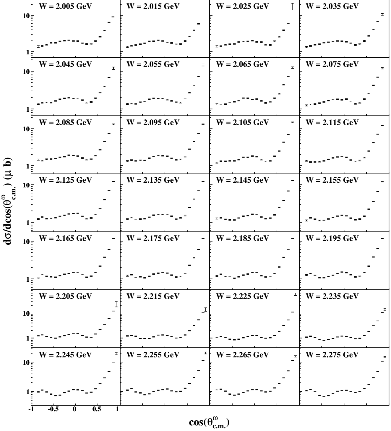
FIG. 8: \frac{d\sigma}{d\cos\theta_{c.m.}^\omega} ( \mu\text{b} ) versus \cos\theta_{c.m.}^\omega : Differential cross-section results for bins in the energy range 2.00 \text{ GeV} \leq W < 2.28 \text{ GeV} . The centroid of each 10-MeV wide bin is printed on the plot. The error bars, which do not include systematic uncertainties, are discussed in the text.
