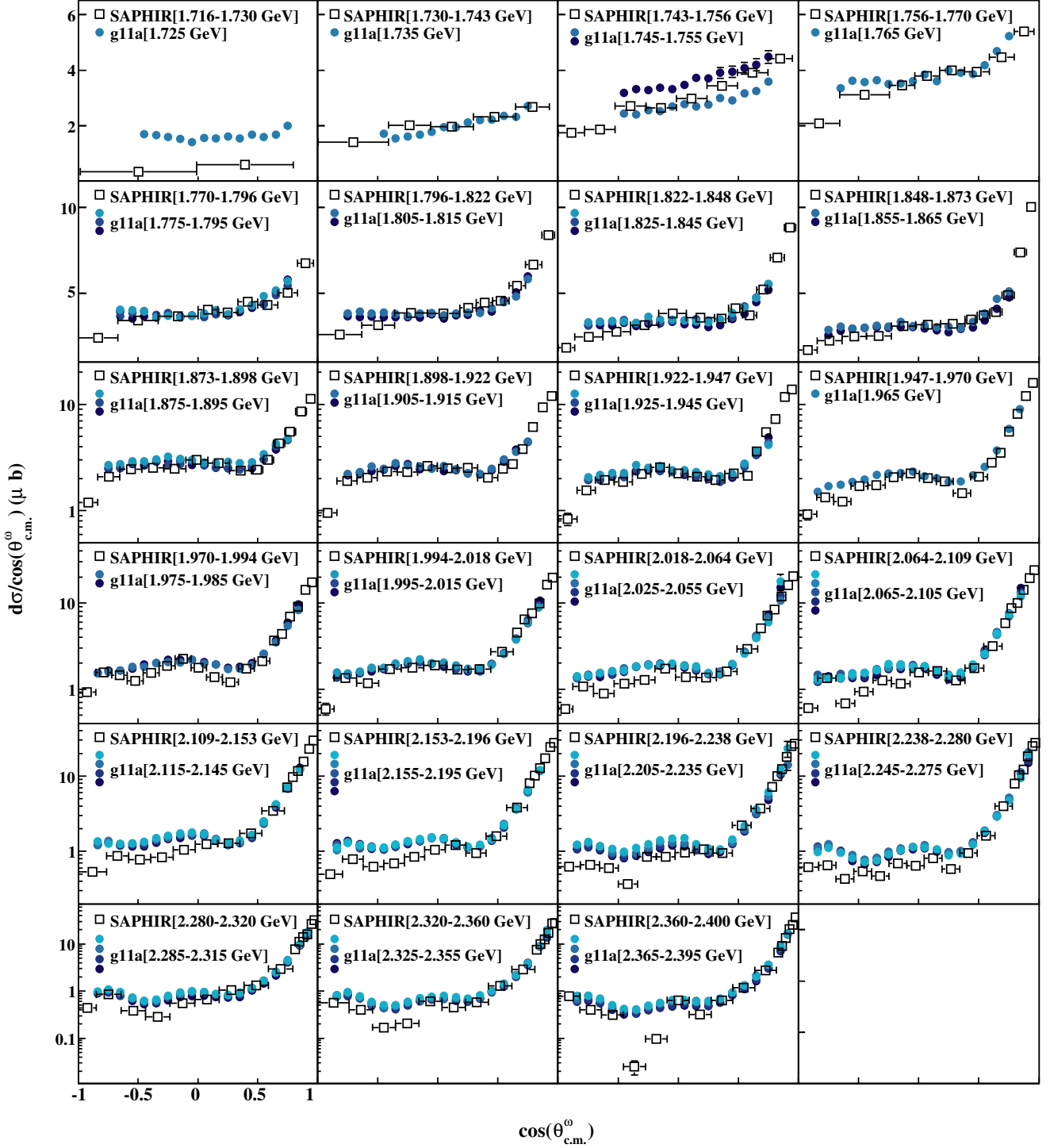
FIG. 17: (Color Online) \frac{d\sigma}{d\cos\theta_{c.m.}^0} ( \mu\text{b} ) versus \cos\theta_{c.m.}^0 : Comparison of the present CLAS results (blue circles) with previously published results from SAPHIR [5] (black open squares).
