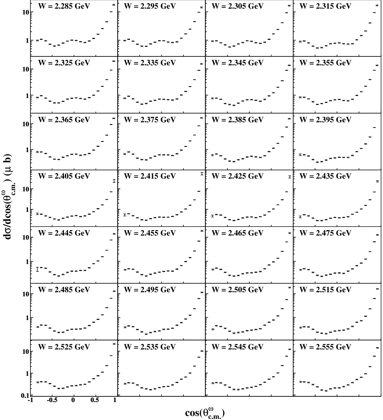
FIG. 9: \frac{d\sigma}{d\cos\theta_{c.m.}^\omega} ( \mu\text{b} ) versus \cos\theta_{c.m.}^\omega : Differential cross-section results for bins in the energy range 2.28\text{ GeV} \leq W < 2.56\text{ GeV} . The centroid of each 10-MeV wide bin is printed on the plot. The error bars, which do not include systematic uncertainties, are discussed in the text.
