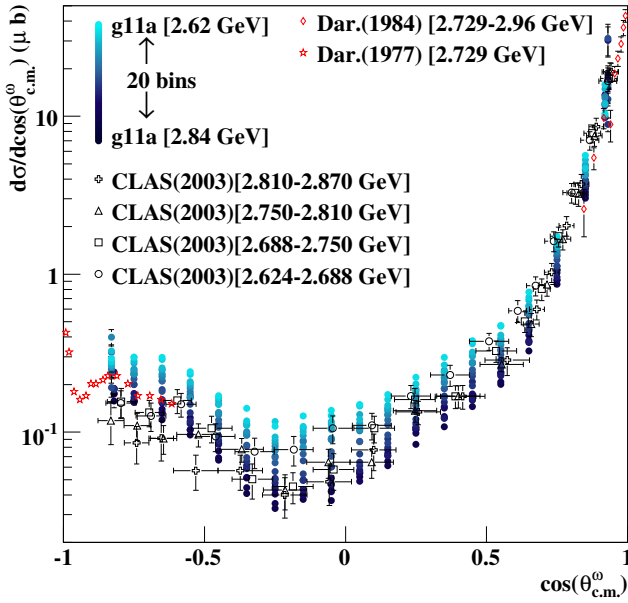
FIG. 16: (Color Online) \frac{d\sigma}{d\cos\theta_{c.m.}^\omega}(\mu b) versus \cos\theta_{c.m.}^\omega : Comparison of the present CLAS results (blue circles) with previously published results from CLAS [4] (black open crosses, triangles, squares and circles) and Daresbury [2, 3] (red open diamonds and stars) in the energy range 2.62 \text{ GeV} < W < 2.96 \text{ GeV} . The Daresbury (1977) points have no error bars; the points were extracted from a portable document format (PDF) image.
