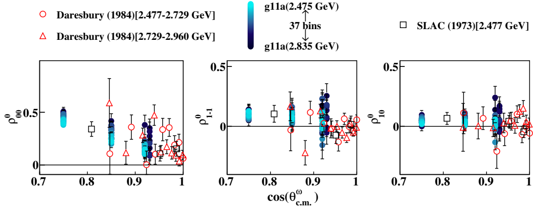
FIG. 19: (Color Online) \rho_{MM'}^0 in the Adair frame versus \cos\theta_{c.m.}^\omega : Comparison of the present CLAS results (blue circles) with previously published Daresbury [3] (open red circles and triangles) and SLAC [1] (open black squares).
